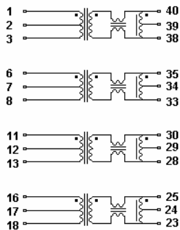
TX 1CT:1CT
