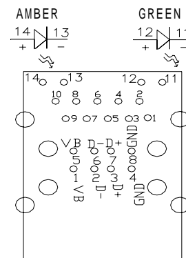
RECOMMENDED P.C.B LAYOUT COMPONENT SIDE OF BOARD
